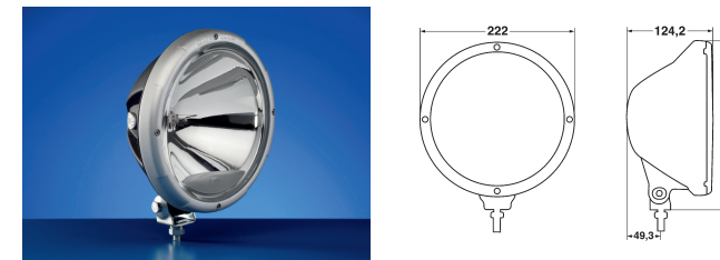
Rallye 3003 – IAM 009 797-021 H: 242mm W: 222mm D: 124.2mm Unique housing design / Latest Lighting technology / High boost reflector / Modern clear glass design also available in cool blue look
