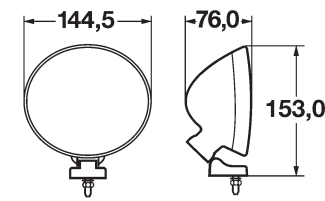
Comet FF 200 Set – IAM 007 893-811 H: 153 mm W: 144,5 mm D: 76 mm Small, round auxiliary light in stylish design / Free-form Reflector / Modern clear-glass design / Also available in cool blue look
