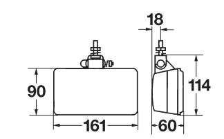
Comet 450 Set – IAM 005 860-831 L: 161 mm H: 114 mm W: 90 mm Light Function with High Beam / Rated Voltage 12 V / Illuminated Area 161 x 90 mm / Housing Colour Black
