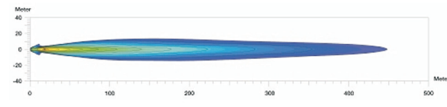
Comet 200 Chromium – IAM 007 893-191 H: 153 mm W: 76 mm D: 144,5 mm Exclusive chrome styling / Classic stylish outfit / Clear-glass design / FF high-gloss reflector / Aluminium vapour-coated reflector
