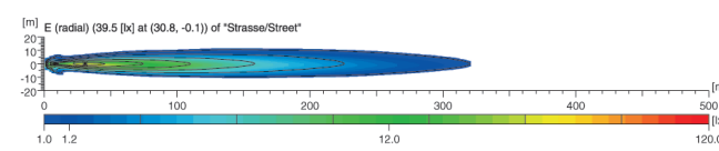
Comet 450 Set – IAM 005 860-831 L: 161 mm H: 114 mm W: 90 mm Light Function with High Beam / Rated Voltage 12 V / Illuminated Area 161 x 90 mm / Housing Colour Black
