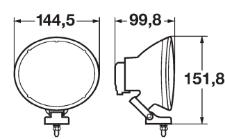
Comet 200 Xenon – IAM 007 893-871 H: 151,8 mm W: 144,5 mm D: 99,8 mm Xenon lighting technology / Elegant Auxiliary light / Free-form reflector with torsion look
