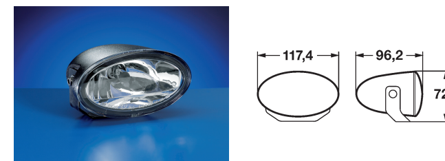
FF 50 – IAM 008 283-801 H: 72.9 mm W: 117.4 mm D: 96.2 mm Compact, Oval Auxiliary Light / Free form magnesium reflectors / Modern clear glass design
