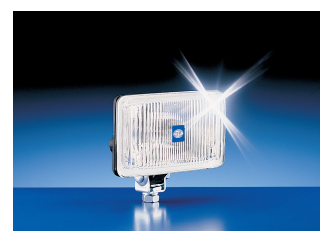
Comet 450 Set – IAM 005 860-831 L: 161 mm H: 114 mm W: 90 mm Light Function with High Beam / Rated Voltage 12 V / Illuminated Area 161 x 90 mm / Housing Colour Black
