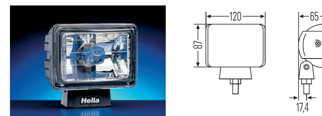
Micro FF Set – IAM 007 133-841 L: 120 mm H: 87 mm W: 65 mm Small and light weight / Sturdy and shock proof design / Rectangular black housing with clear lens design / Easy mounting adjustment and bulb replacement
