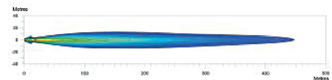
Comet FF 200 Set – IAM 007 893-811 H: 153 mm W: 144,5 mm D: 76 mm Small, round auxiliary light in stylish design / Free-form Reflector / Modern clear-glass design / Also available in cool blue look
