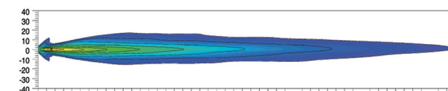
Rallye 4000 – IAM 007 560-121 H: 232.5 mm W: 129.6 mm D: 224.4 mm High-quality diecast zinc housing / Reflector glued to lens. Sulphur-treated lens / Black lens frame and housing / With bracket installed and built-in 12 V/100 W bulb / For upright or suspended installation
