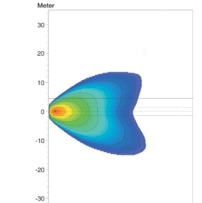
Premium Light Micro DE Set – IAM 008 090-821 H: 90mm W: 90mm D: 94.2 mm Smallest auxiliary light from HELLA / Reflector and housing made of high-grade metal materials / Sophisticated aluminium design housing
