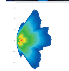
Dyna View Evo 2 Set – IAM 009 295-801 H: 90 mm W: 94.2 mm D: 90 mm CORNERING LIGHT DynaView Evo2 system / Combines the safety functions of cornering light and fog light in compact, round auxiliary lights / When the dipped beam is on the left or right cornering light will automatically turn itself on without a delay when the indicator is set or when the car drives through a curve at no more than 40kmh
