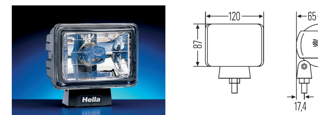
Micro FF – IAM 007 133-851 L: 120 mm H: 87 mm W: 65 mm Small and light weight / Sturdy and shock proof design / Rectangular black housing with clear lens design / The latest aluminium vapour coated free form reflector for precise and optimum light output, Illumination upto 300 m / Easy mounting adjustment and bulb replacement
