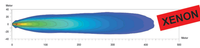
Comet 200 Xenon – IAM 007 893-871 H: 151,8 mm W: 144,5 mm D: 99,8 mm Xenon lighting technology / Elegant Auxiliary light / Free-form reflector with torsion look
