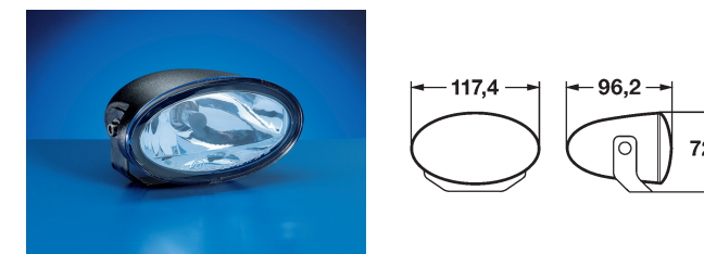
FF 50 Blue Set – IAM 008 283-861 L: 117.4 mm H: 96.2 mm W: 72.9 mm Modern clear lens design / Free-form (FF) reflector / Black housing color / Oval Design / Suitable for upright and pendant flush-fitting
