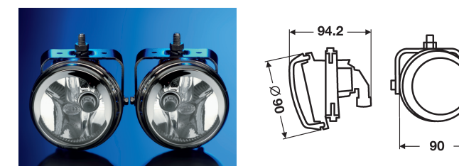
Dyna View Evo 2 Set – IAM 009 295-801 H: 90 mm W: 94.2 mm D: 90 mm CORNERING LIGHT DynaView Evo2 system / Combines the safety functions of cornering light and fog light in compact, round auxiliary lights / When the dipped beam is on the left or right cornering light will automatically turn itself on without a delay when the indicator is set or when the car drives through a curve at no more than 40kmh
